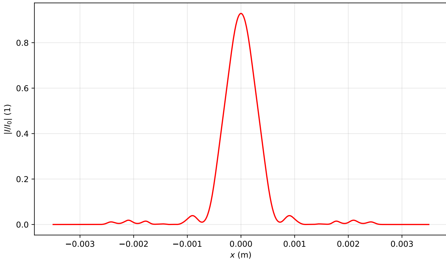
Intensity profile I(x, y = 0, z = 3.344)/I_0 , \text{Pin}=2.0\text{Pcr} , artificial time
